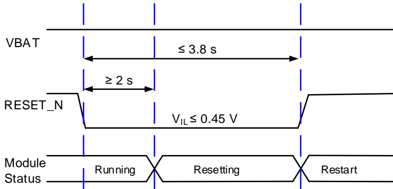
Figure 17: Reset Timing
