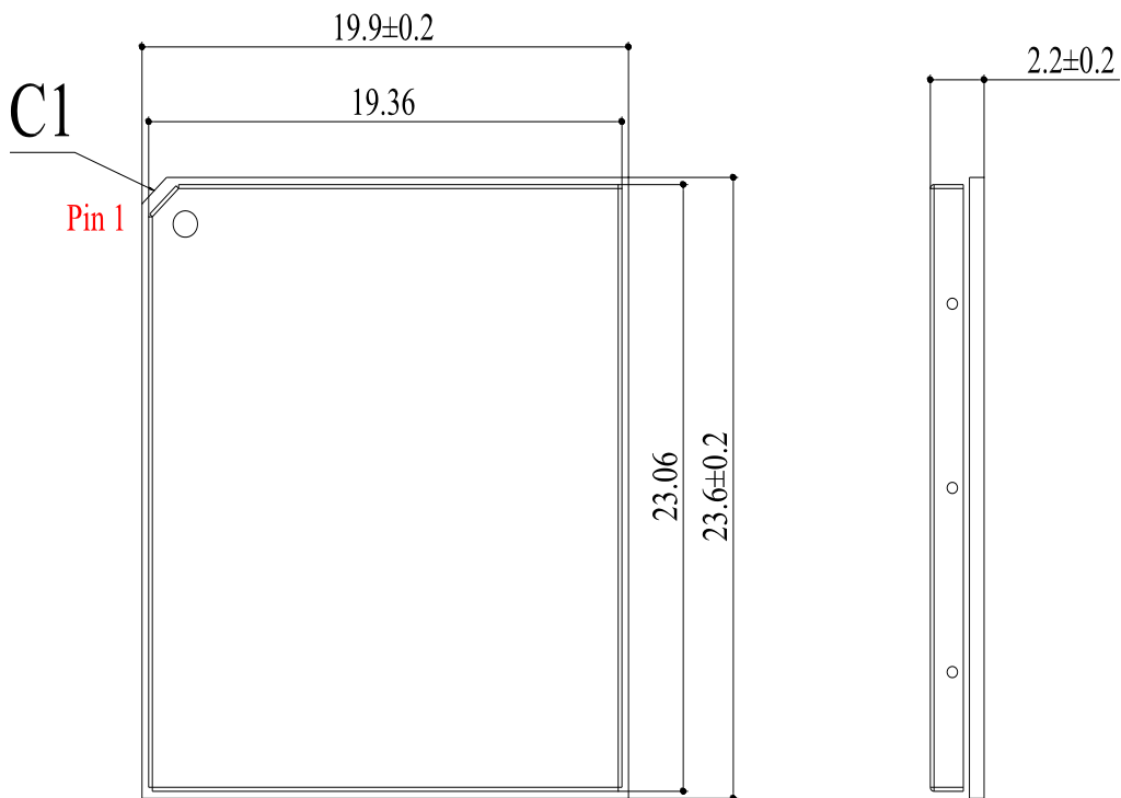
Figure 42: Module Top and Side Dimensions
