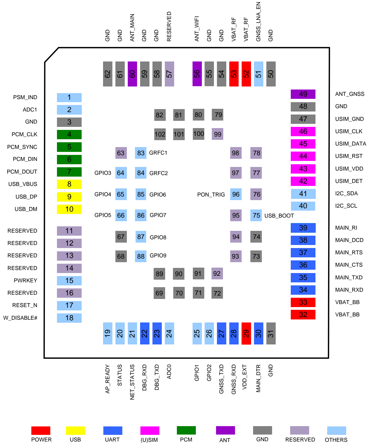
Figure 8: Pin Assignment (Top View)
