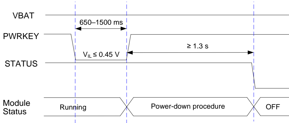
Figure 15: Power-down Timing
