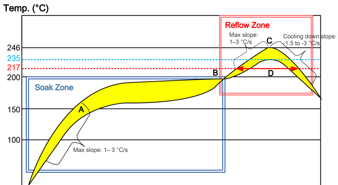
Figure 38: Recommended Reflow Soldering Thermal Profile
