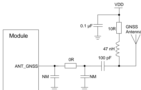
Figure 26: Reference Design of GNSS Antenna Interface
