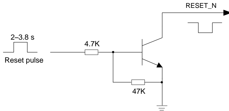
Figure 10: Reference Design of RESET_N with a Driving Circuit
