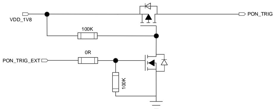
Figure 13: Reference Design of PON_TRIG
