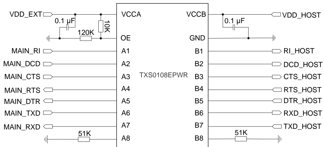
Figure 18: Main UART Reference Design (IC Solution)
