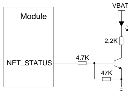
Figure 21: Reference Design of NET_STATUS
