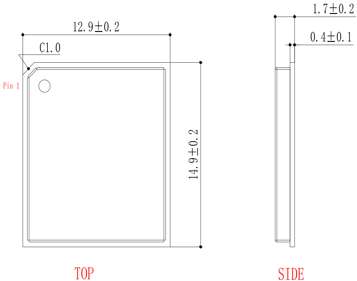
Figure 34: Module Top and Side Dimensions
