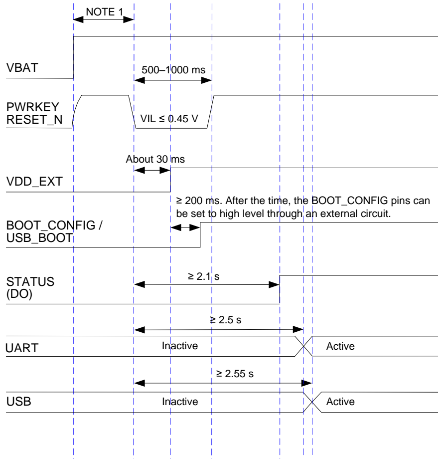
Figure 7: Power-up Timing
