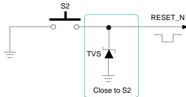
Figure 11: Reference Design of RESET_N with a Button
