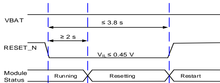
Figure 12: Reset Timing
