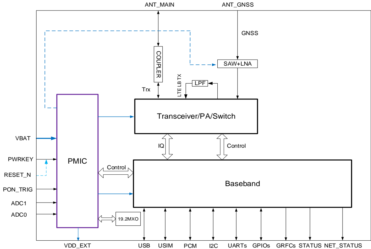
Figure 1: Functional Diagram
