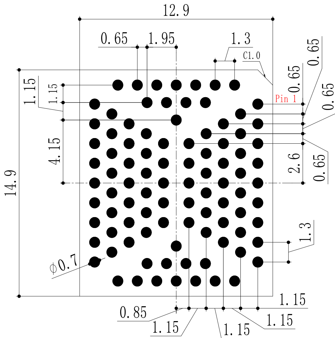
Figure 35: Module Bottom Dimensions (Bottom View)
