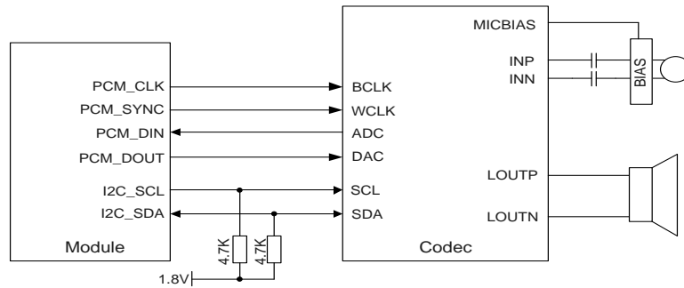
Figure 20: Reference Design of PCM Application with Audio Codec
