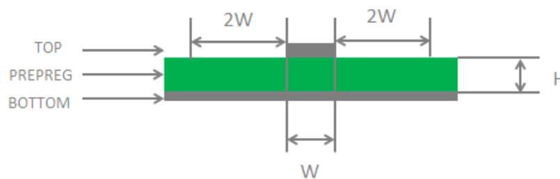
Figure 27: Microstrip Design on a 2-layer PCB
