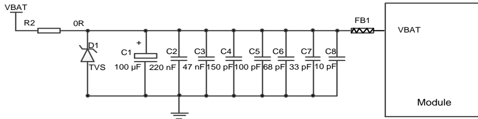
Figure 4: Reference Design of Power Supply
