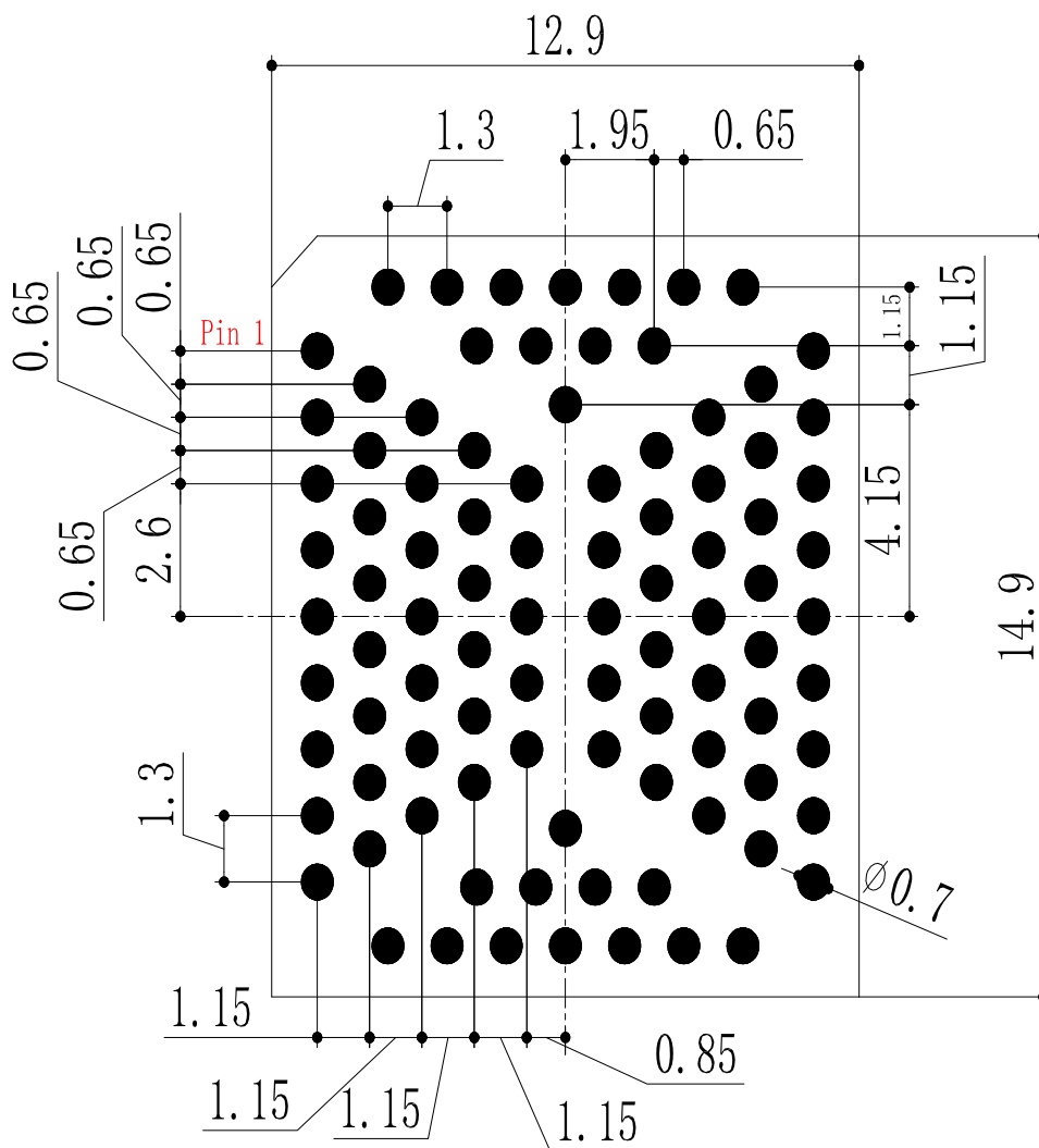
Figure 36: Recommended Footprint (Top View)
