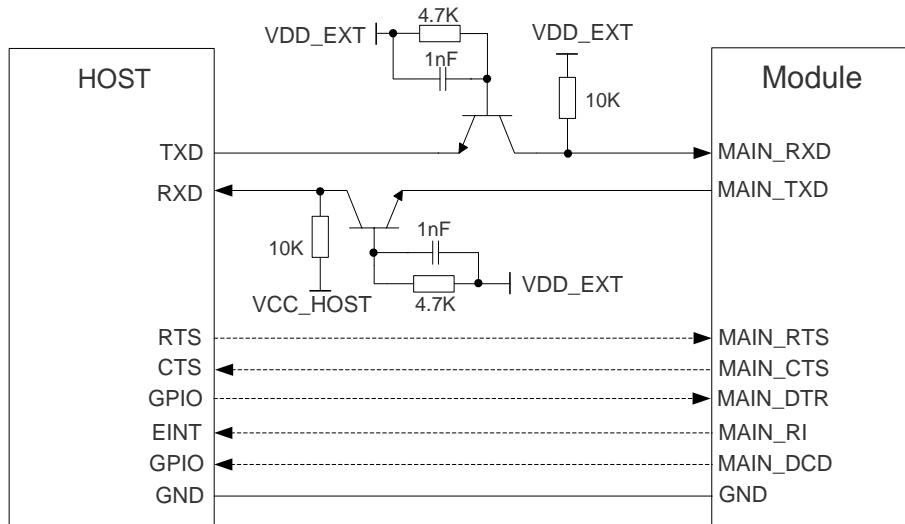
Figure 19: Main UART Reference Design (Transistor Solution)
