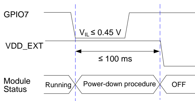
Figure 9: Fast Shutdown Timing
