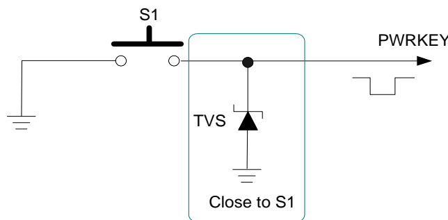
Figure 6: Turn on the Module with a Button
